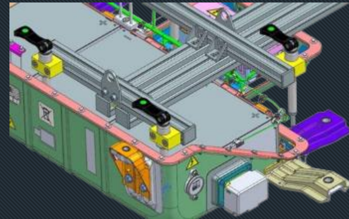
Prototype for tools that remove modules from electric batteries.
